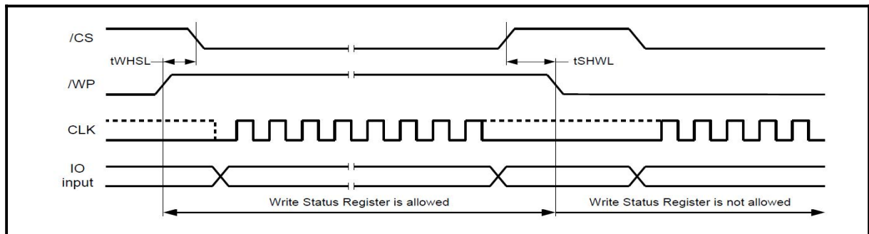
Figure 48. /WP Timing
