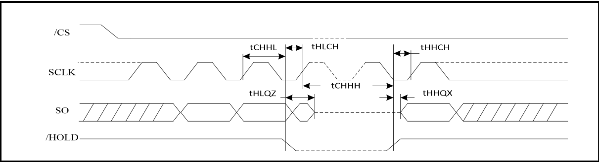
Figure 171. /WP Timing
