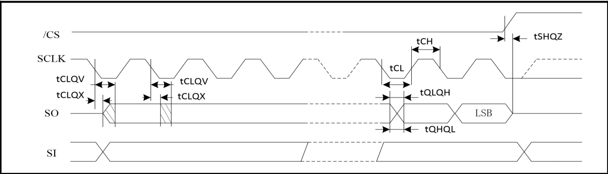
Figure 170. Hold Timing
