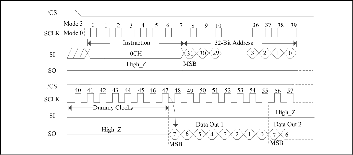
Figure 40. Fast Read with 4-Byte Address
