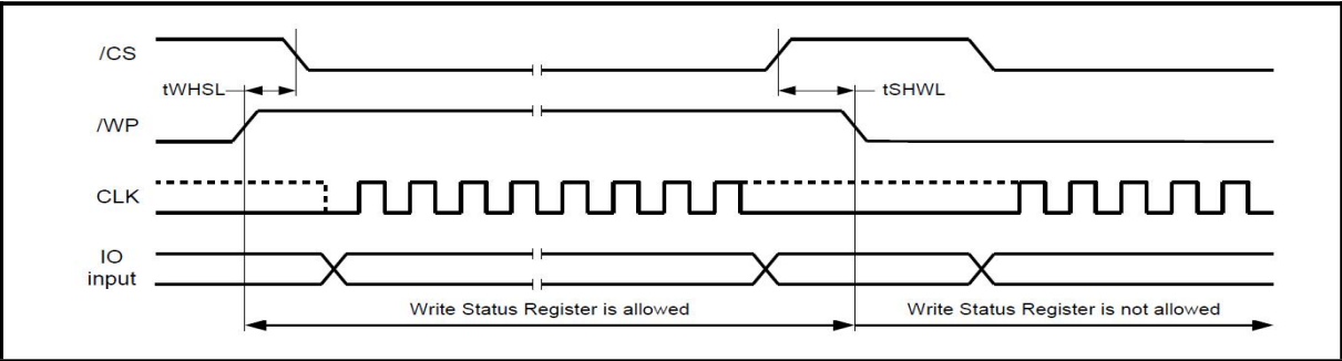
Figure 172. DQS Output Timing (DTR)
