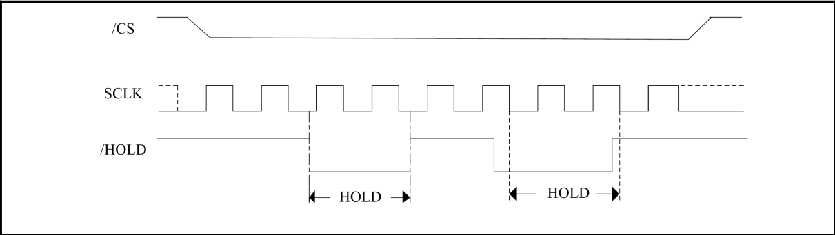
Figure 6. Hold condition activation
