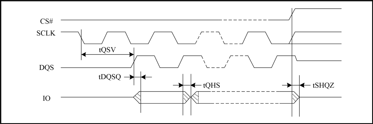
Figure 173. DQS Output Timing (Non DTR)
