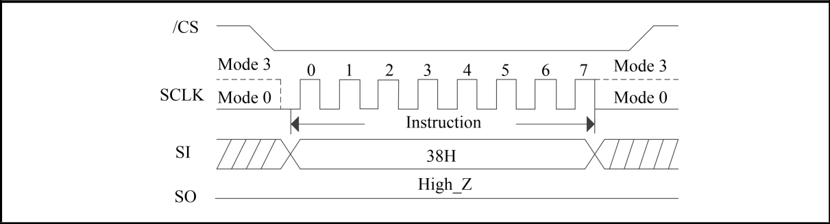
Figure 29. Enter QPI Mode (SPI Mode)
