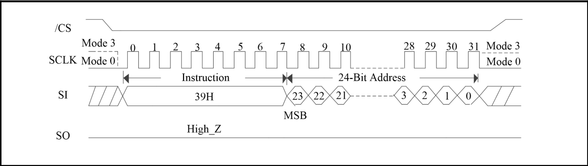
Figure 158. Individual Block/Sector Unlock (SPI Mode/4-Byte Address Mode)
