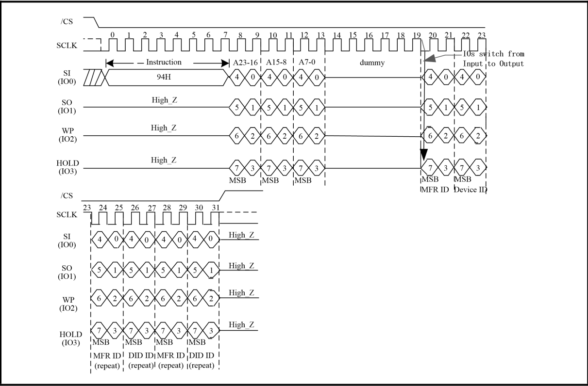
Figure 88. Quad I/O Read Manufacture ID/ Device ID Sequence Diagram (SPI Mode/3-Byte Address Mode)
