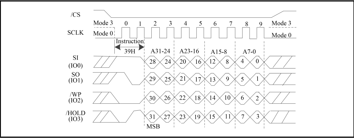
Figure 160. Individual Block/Sector Unlock (QPI Mode/4-Byte Address Mode)
