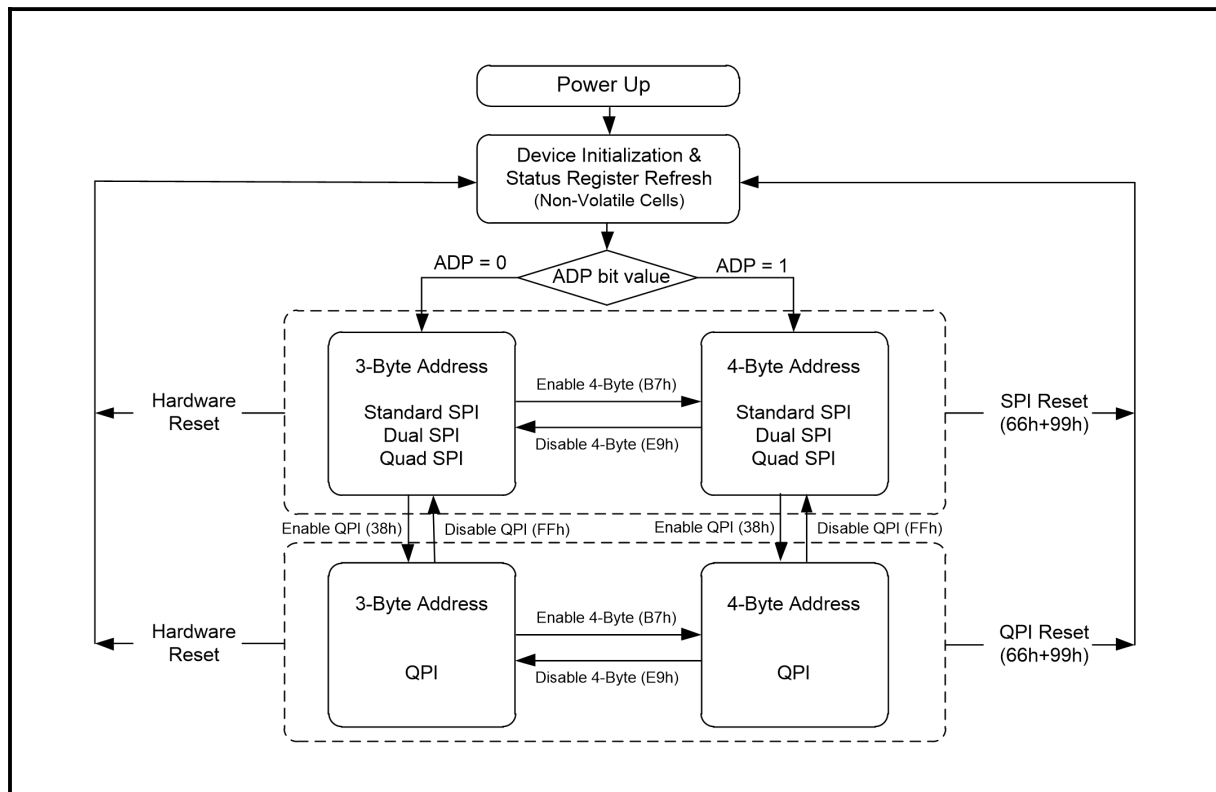
Figure 5. BY25FQ256ES Serial Flash Memory Operation Diagram
