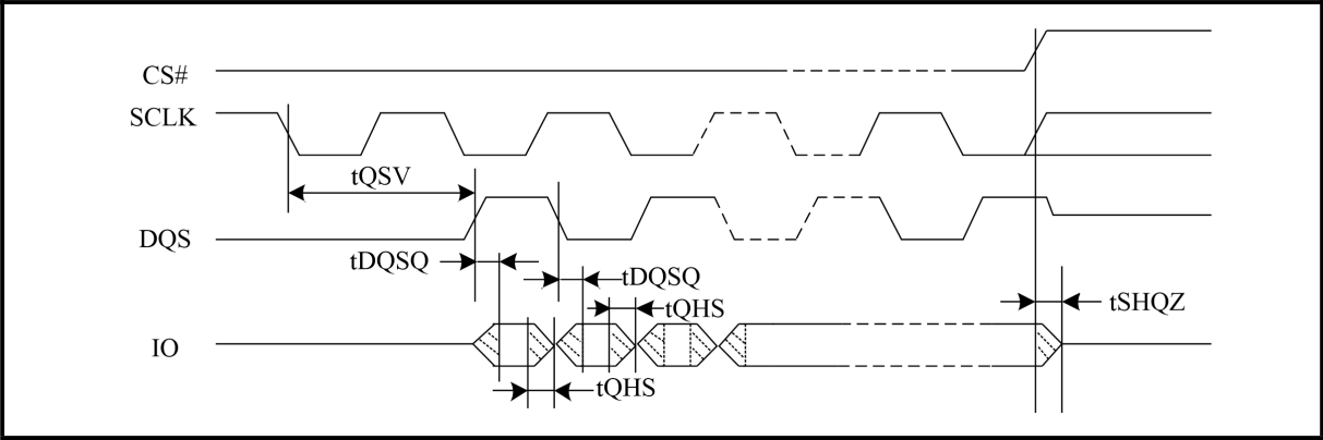
Figure 173. DQS Output Timing (Non DTR)
