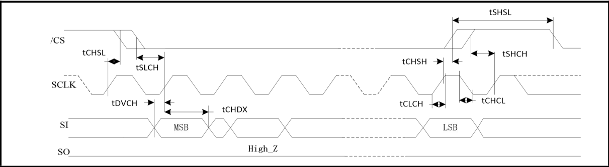
Figure 169. Output Timing
