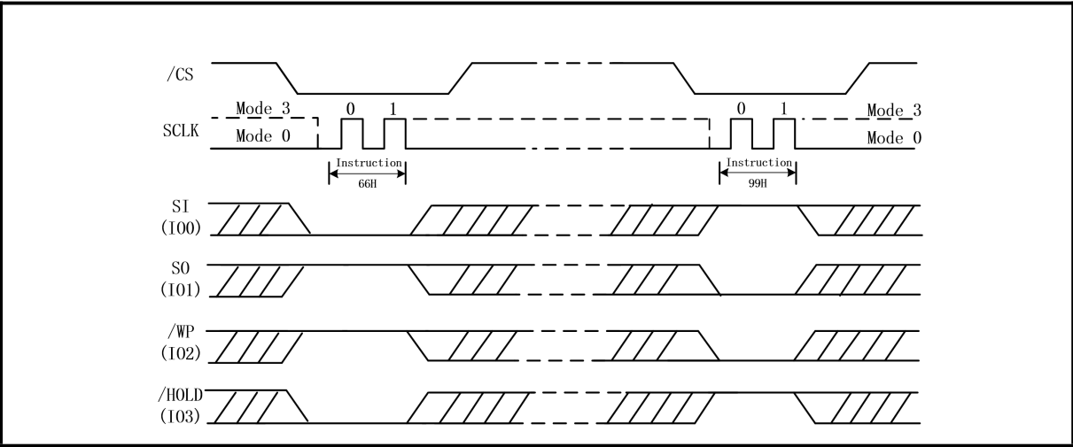
Figure 32. Enable Reset (66h) and Reset (99h) Instruction Sequence (QPI Mode)
