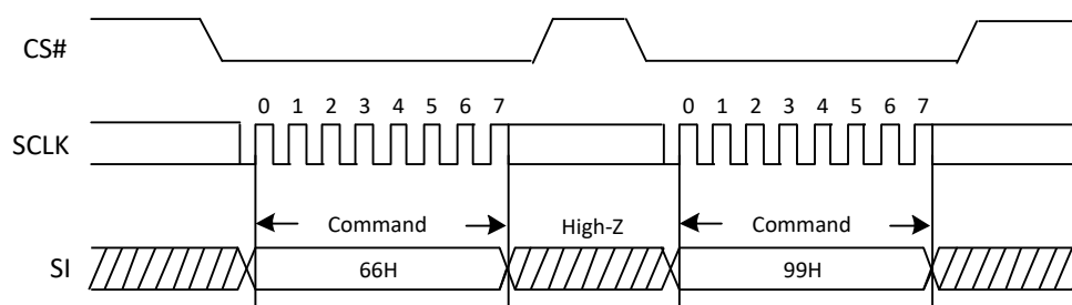
Figure 29. Enable Reset and Reset command Sequence Diagram
