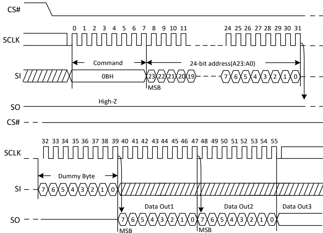
Figure 8. Read Data Bytes at Higher Speed Sequence Diagram
