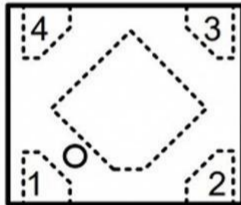
DFN1X1-4
